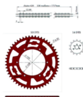
Chain Kit aluminium red 14x53 - 420 Doppler Derbi GPR / Aprilia
